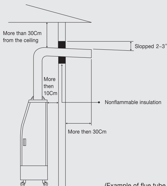
(Example of flue tube installation)
