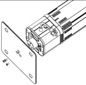
Figure1: Assembly diagram of the base
